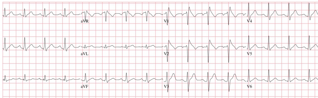
Figure 15. Brugada Syndrome
